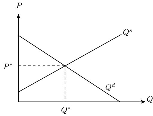
Figure 1: Supply and demand.
